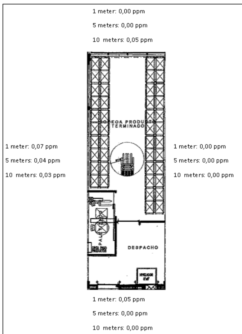
Figure 3. Ambient concentration around the fumigated warehouse during exposure time.
