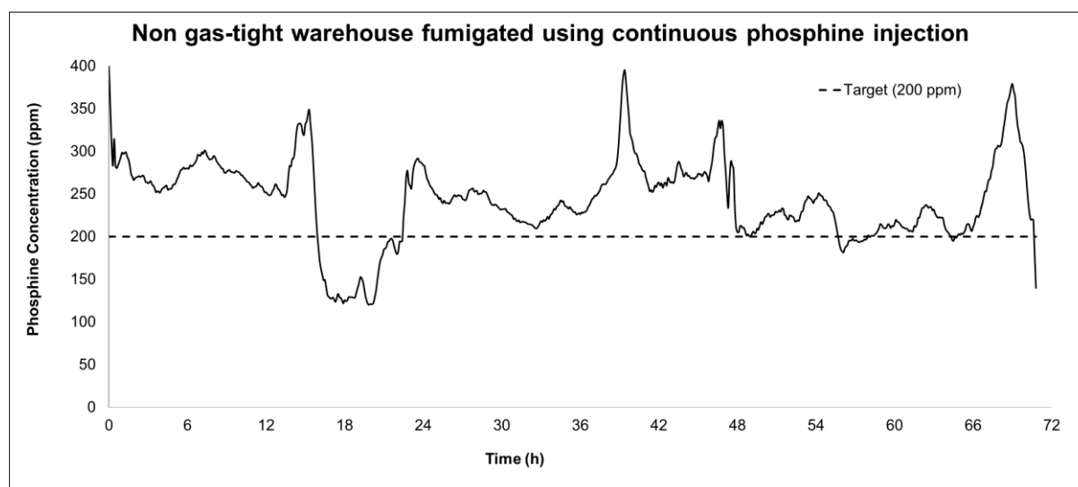
Figure 1. Phosphine concentration record obtained from the non gas-tight warehouse fumigated using continuous phosphine injection.
