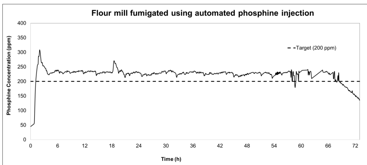
Figure 2. Phosphine concentration record obtained from the flour mill fumigated using automated phosphine injection.
